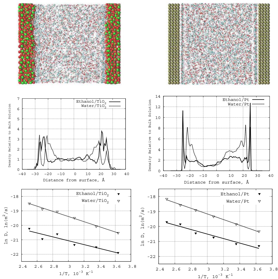
Fig. (7). Top: Snapshots of the ethanol-water mixture in the presence of TiO 2 (left) and Pt (right) surfaces. Middle: Z-density distributions of ethanol (solid line) and water (dashed line) on the TiO 2 (left) and Pt (right) surfaces. Bottom: Relation between \ln D(T) and reciprocal temperature in Kelvin: ethanol (solid line) and water (dashed line) in the presence of TiO 2 (left) and Pt (right) surfaces.
