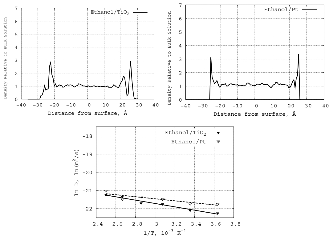
Fig. (6). Top: Z-density distributions of pure ethanol on the TiO 2 (left) and Pt (right) surfaces. Bottom: Relation between \ln D(T) and reciprocal temperature in Kelvin; ethanol in the presence of TiO 2 (solid line) and Pt (dashed line) surfaces.
