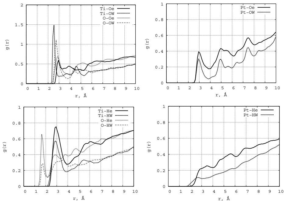
Fig. (9). RDF for ethanol (Oe, He) and water (OW, HW) atoms on the TiO 2 (left) and Pt (right) surfaces.
