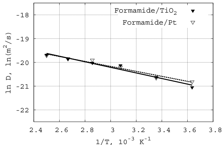
Fig. (2). Relation between \ln D(T) and reciprocal of temperature in Kelvin; solid line for formamide on TiO 2 (anatase) and dashed line for formamide on Pt (platinum) surfaces.
