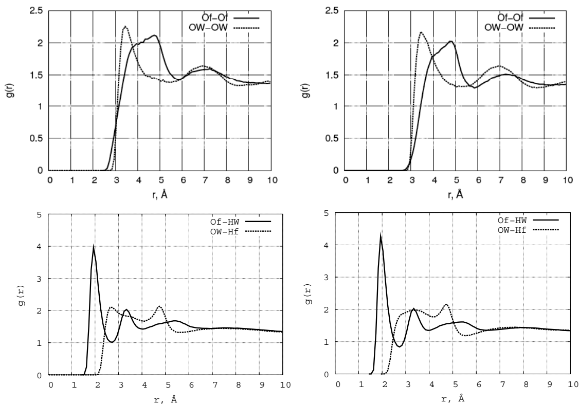
Fig. (4). The radial distribution functions (RDF) for Of-Of, OW-OW, Of-HW, and OW-Hf of the formamide–water mixture interacting with the TiO 2 (left) and Pt (right) surfaces.
