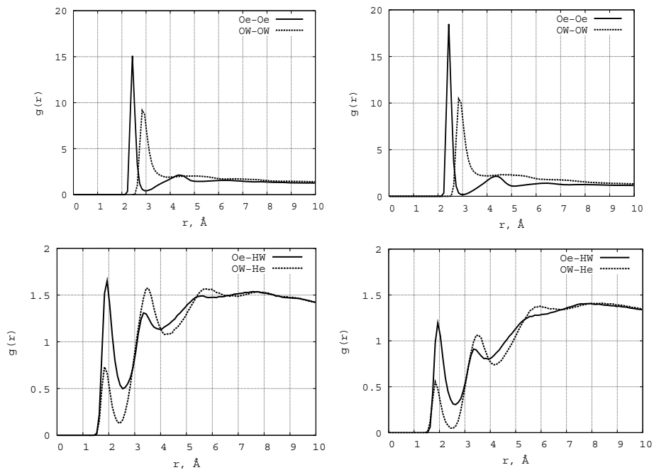
Fig. (8). The RDF for Oe-Oe, OW-OW, Oe-HW, and OW-He of the ethanol-water mixture on the TiO 2 (left) and Pt (right) surfaces.
