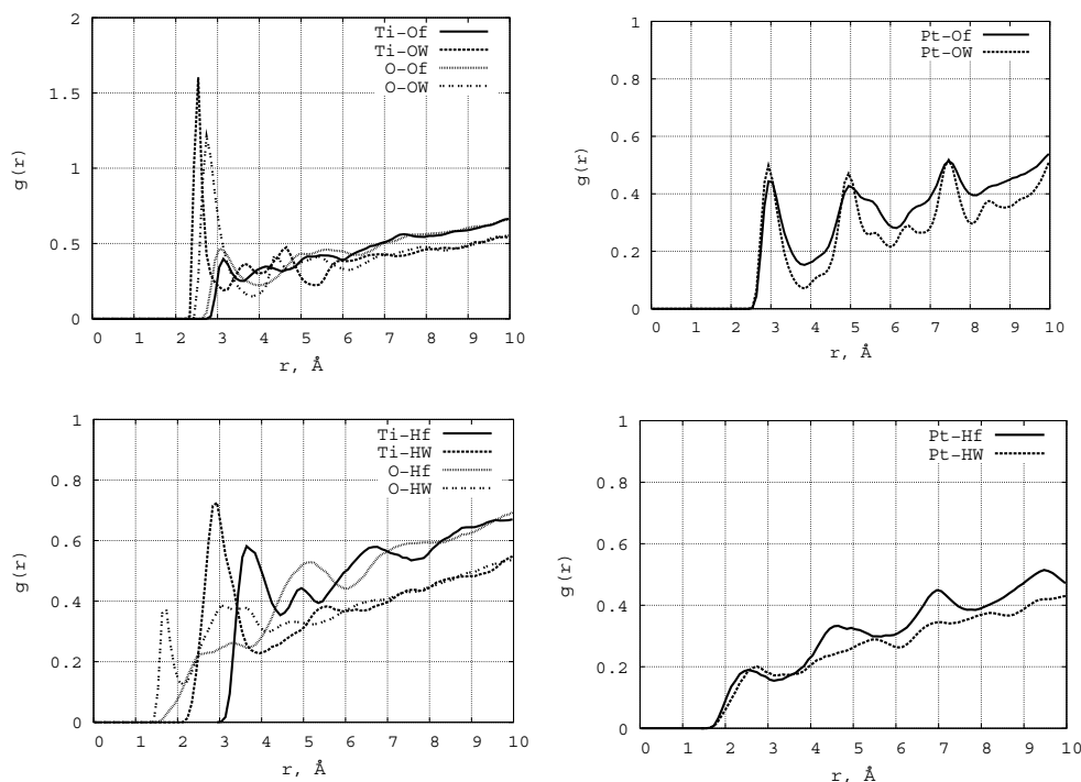
Fig. (5). The RDF for the formamide (Of, Hf) and water (OW, HW) atoms on the \text{TiO}_2 (left) and Pt (right) surfaces.
