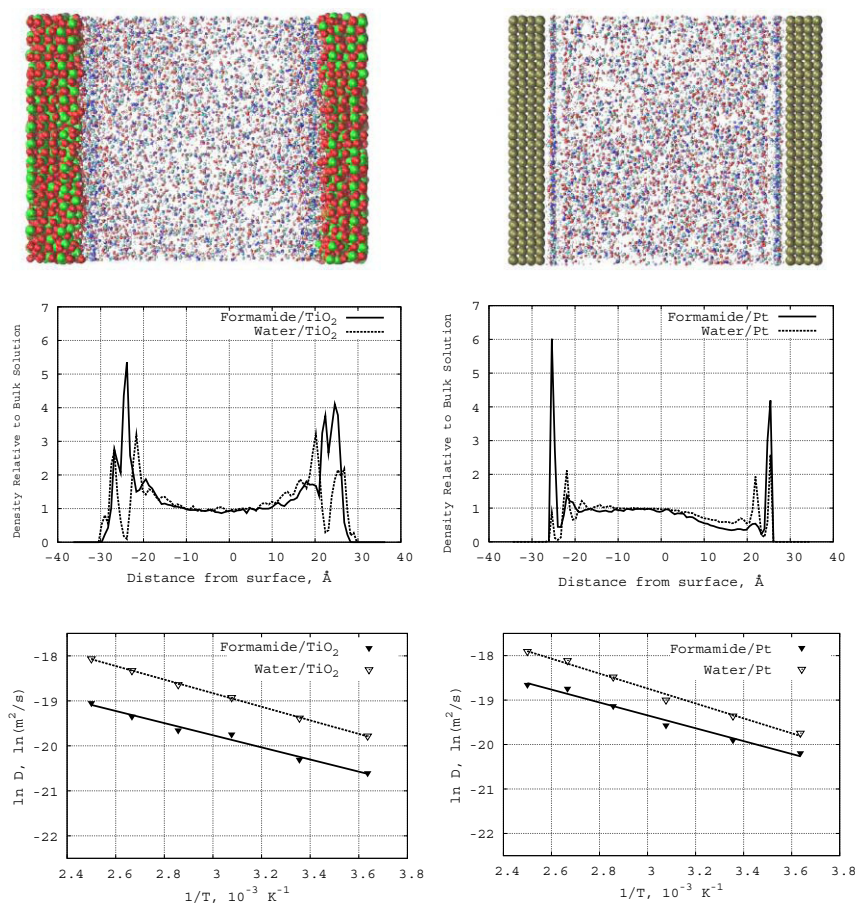
Fig. (3). Top: Snapshots of a formamide–water mixture in the presence of TiO 2 (anatase; left) and Pt (platinum; right) surfaces. Middle: Z-density distributions of formamide (the solid line) and water (the dashed line) on the TiO 2 (left) and Pt (right) surfaces. Bottom: The relation between \ln D(T) and reciprocal temperature in Kelvin; the solid line is for formamide and the dashed line is for water in the presence of TiO 2 (left) and Pt (right) surfaces.
