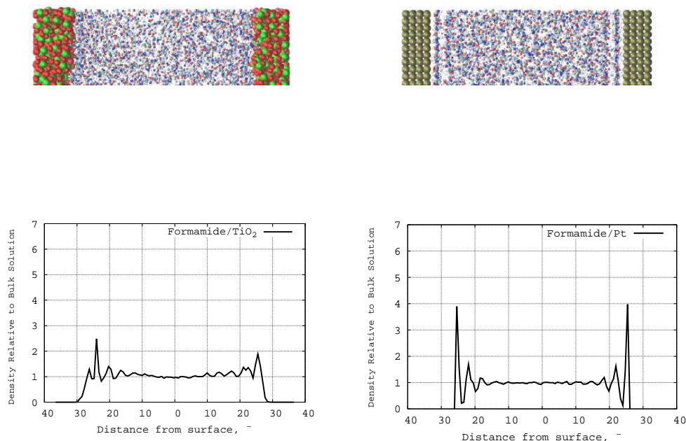
Fig. (1). Top: snapshots of pure formamide in the presence of TiO 2 (left) and Pt (right) surfaces. Bottom: Z-density distributions of pure formamide on the TiO 2 (left) and Pt (right) surfaces.
