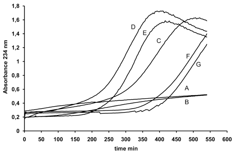
Fig. (1). Cu 2+ catalysed LDL peroxidation: antioxidant and prooxidant effect of coffee.
