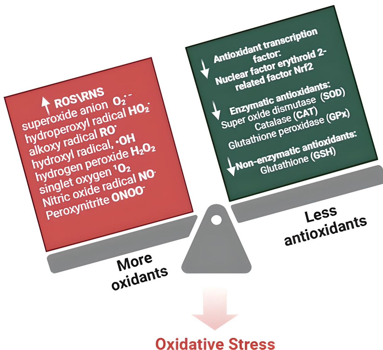
Fig. (1). Factors influencing redox imbalance and key oxidative stress markers, highlighting the relationship between reactive oxygen species (ROS), reactive nitrogen species (RNS), and antioxidant defenses in cellular homeostasis. Adapted and modified from [5].
