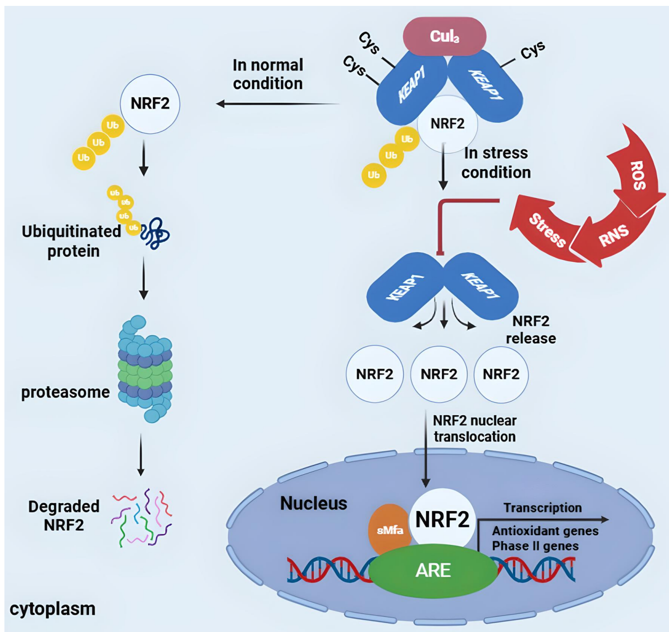
Fig. (2). The Keap1-Nrf2-ARE signaling pathway. Under basal conditions, Keap1 inhibits Nrf2 by promoting its degradation. Upon oxidative stress, Nrf2 dissociates from Keap1, translocates to the nucleus, and activates antioxidant genes (e.g., SOD, CAT, GSH, HO-1) to counteract oxidative damage. Adapted and modified from [11].
